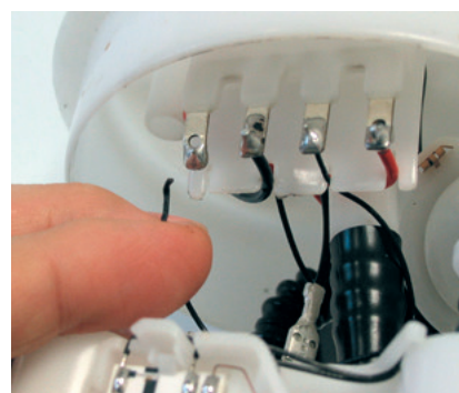
Fig. 3: Typical damage symptoms: the sender unit's cable is detached and the electrical contacts are bent.
